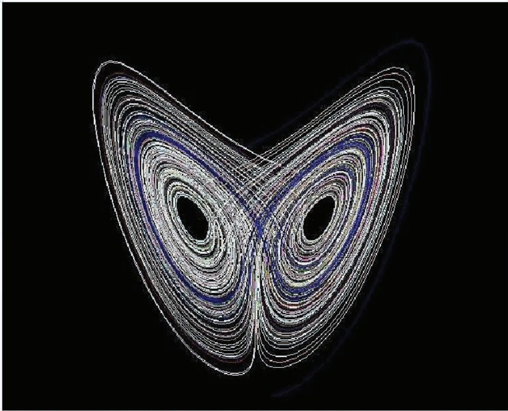
Figure 1- The Lorenz attractor (for dt=0.02 , a=5 , b=15 , c=1 ).
